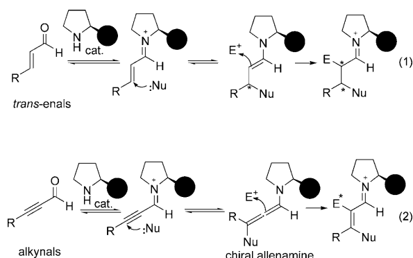
Scheme 1. Conventional (1) and iminium–allenamine (2) catalytic enantioselective iminium-initiated cascade reactions.
