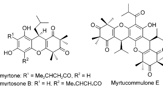
Scheme 2. Examples of 4 H -chromenes as substructures in biologically interesting natural products.
